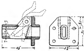
Figs. 718-720. Latch for Damper Handle.
